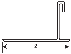
2" closure plate
