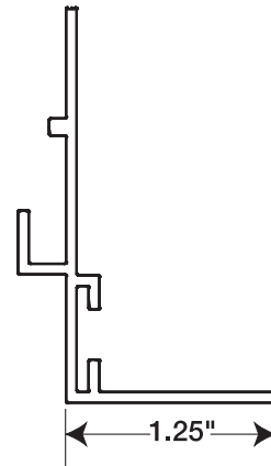
Closure mount with tile support
