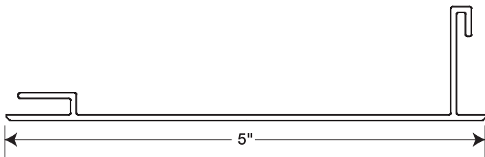
5 inch closure plate
